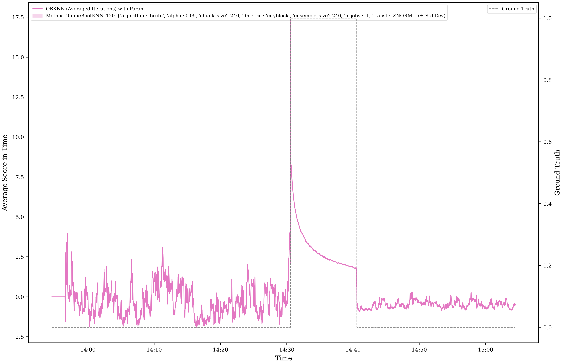
Method OBKNN Score for Scenario A9
